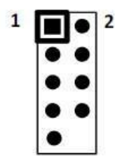
Figure 7: Front Panel Header
