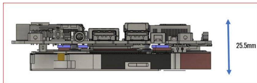
Figure 10: Motherboard w/ Cooler Height Dimensions (Max)
