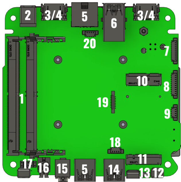
Figure 5: Bottom Side Header Locations
