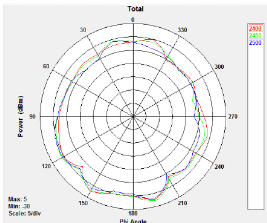
2.4GHz Azimuth-Plane
