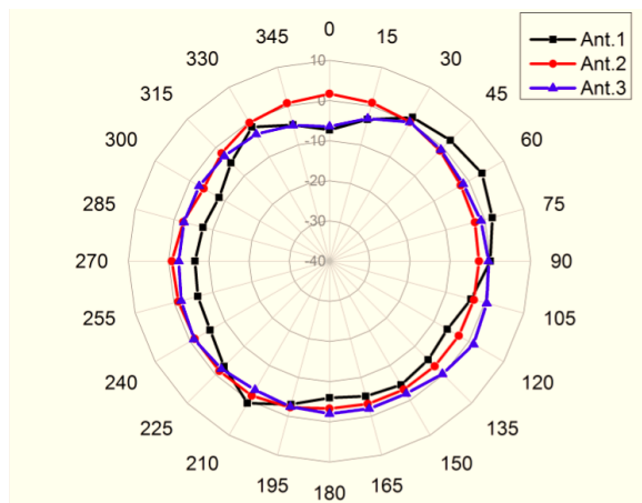
2.4GHz Azimuth-Plane
