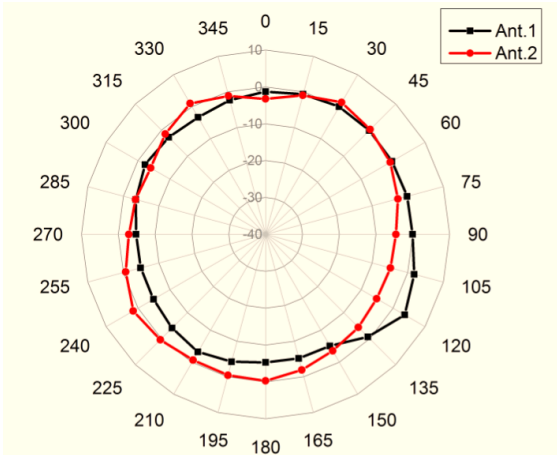
2.4GHz Elevation-Plane
