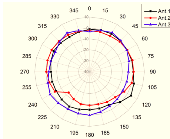
2.4GHz Elevation-Plane
