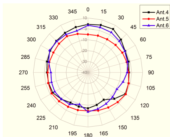
5GHz Elevation-Plane
