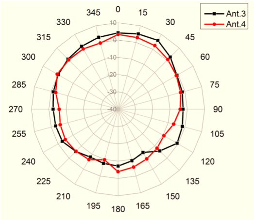
5GHz Elevation-Plane
