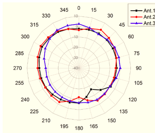
2.4GHz Elevation-Plane
