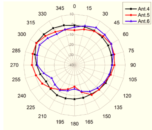
5GHz Elevation-Plane
