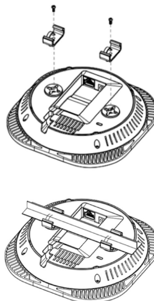
Mounting the AP to a T-Bar
