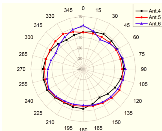
5GHz Azimuth-Plane
