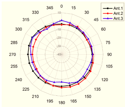
2.4GHz Azimuth-Plane
