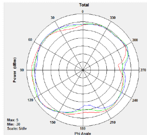
2.4GHz Elevation-Plane
