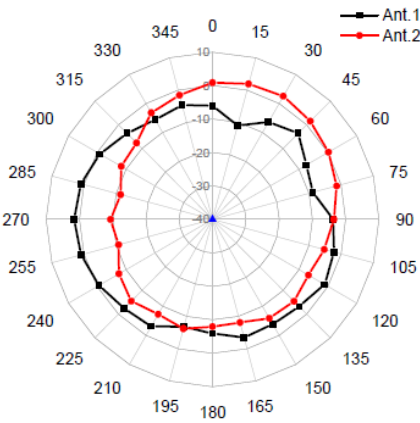
2.4GHz Azimuth-Plane
